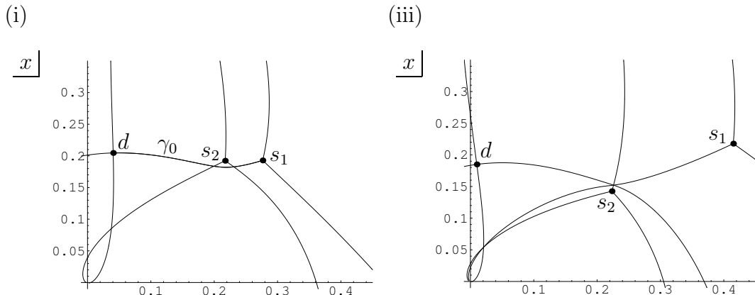
Fig. 2 : Configuration of Stokes curves of (LNY)_2 for (i) t_1 = -1.6104 - 0.2268\sqrt{-1} and (iii) t_3 = -1.5783 - 0.4130\sqrt{-1} .
