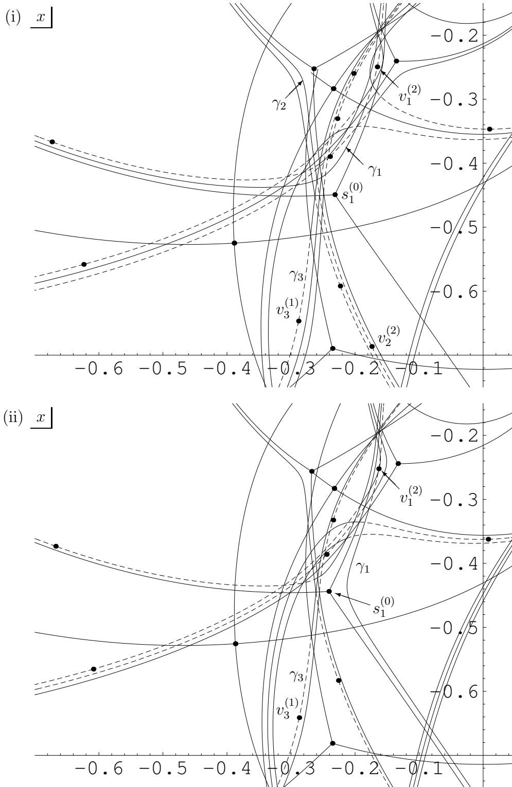
Fig. 9 : Configuration of Stokes curves of (LNY)_4 for (i) t_1 , i.e. in the waking region of v_2^{(2)} , and (ii) t_6 , i.e. in the sleeping region of v_2^{(2)} .
