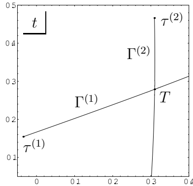
Fig. 4 : Crossing of two Stokes curves \Gamma^{(1)} and \Gamma^{(2)} of (NY)_4 emanating respectively from \tau^{(1)} = -0.0347 + 0.1545\sqrt{-1} and \tau^{(2)} = 0.3094 + 0.4662\sqrt{-1} .
