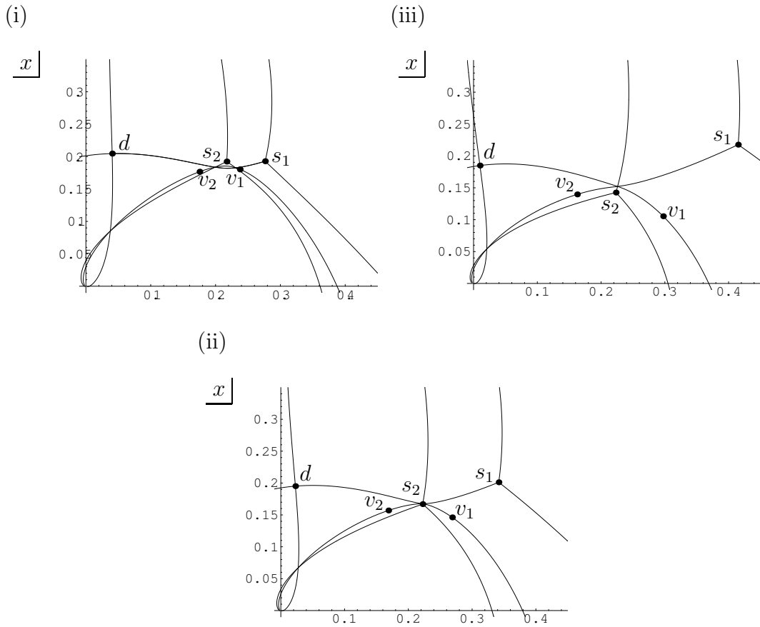
Fig. 3 : Stokes geometry of (LNY)_2 with virtual turning points added. (Figure (i) is for t = t_1 , (ii) for t = t_2 and (iii) for t = t_3 .)
