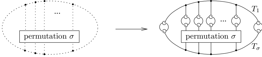
FIGURE 6.3. The connected trivalent diagram \Gamma_\sigma , and the two simple linear C_n^a -trees T_0 and T_\sigma .
