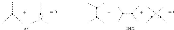
FIGURE 5.1. The AS and IHX relations.
