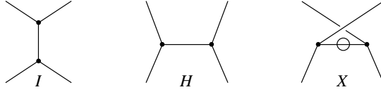
FIGURE 2.7. The three Y_k -graphs I , H and X .
