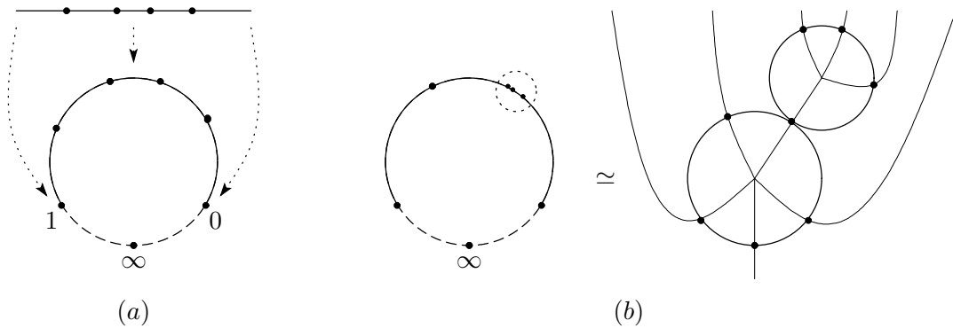
Figure 2: (a). The identification of the interval with n - 2 points on it with the boundary of the disk with n + 1 points on the boundary. (b). The correspondence of the compactification of the moduli spaces with tree graphs; the case of a boundary component of the compactified moduli space \mathcal{M}_7 .
