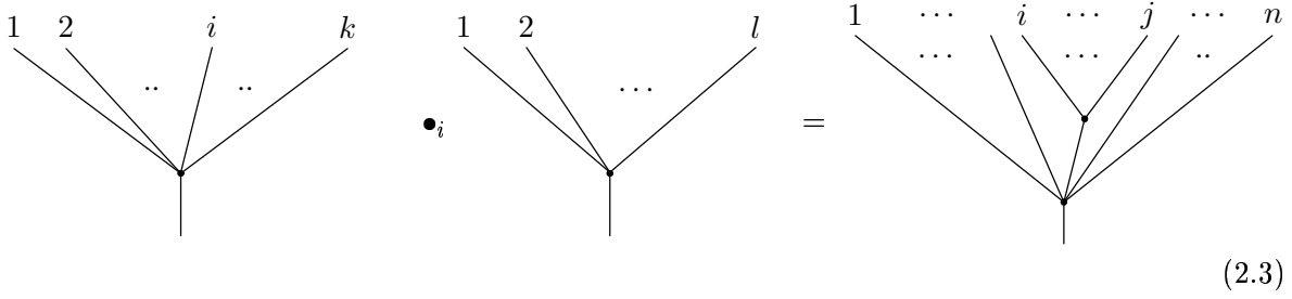
Figure 3: The grafting M_k \bullet_i M_l of the l -corolla M_l to the i -th leaf of k -corolla M_k , where j = i + l - 1 and n = k + l - 1 .
