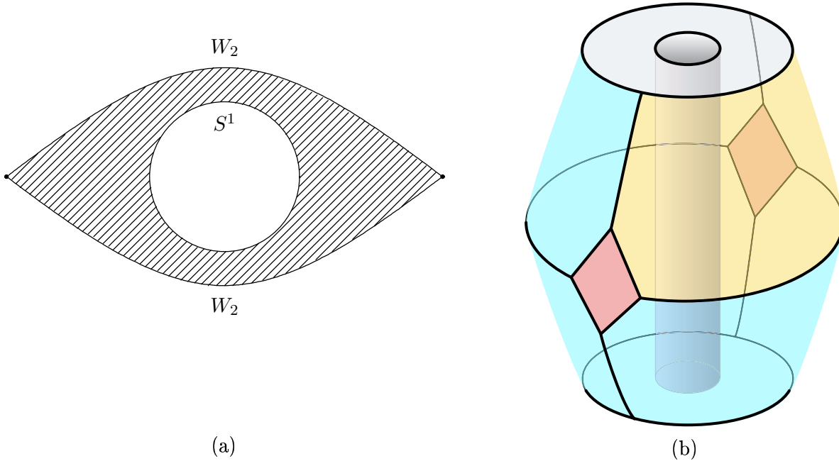
Figure 6: (a): The Eye. (b): The solid torus.
