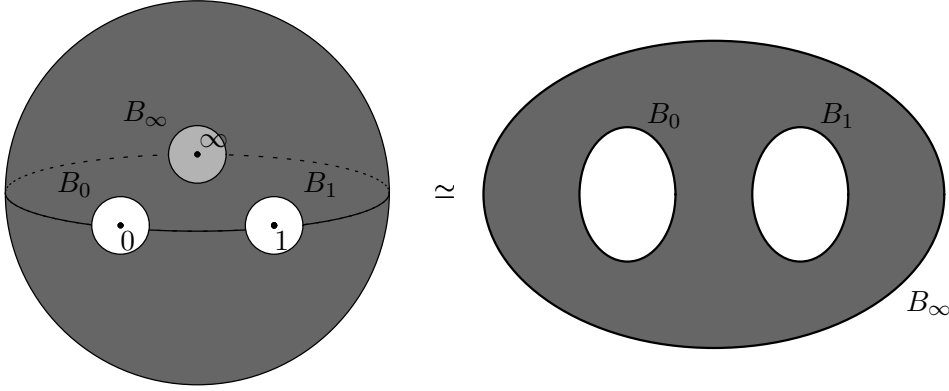
Figure 5: The real compactification \underline{\mathcal{M}}_{0,3+1} of \mathcal{M}_{0,3+1} .
