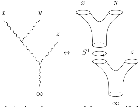
Figure 5: The real compactification \underline{\mathcal{M}}_{0,3+1} of \mathcal{M}_{0,3+1} .
