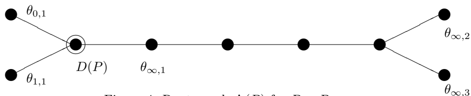
Figure 4: Root graph \Delta(P) for P = P_3
