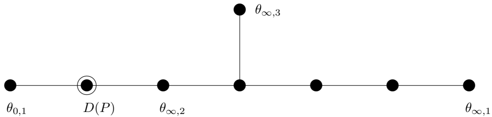
Figure 3: Root graph \Delta(P) for P = P_1
