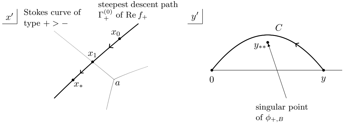
Figure 2. Integration path of (3.6) when y \geq \hat{y} .
