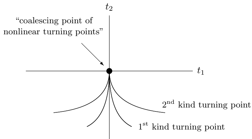
Figure 3. The set of turning points of the fourth order PI equation (P_1)_2
