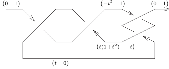
Figure 2: A general non-trivial X_q -coloring of a diagram of the figure-eight knot
