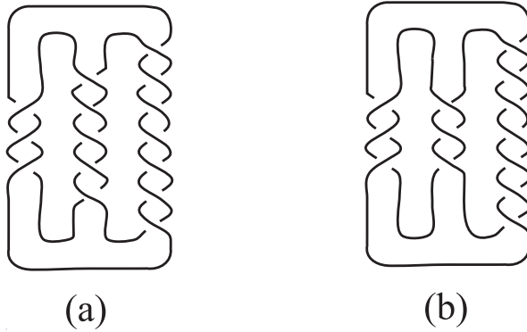
Figure 4: The pretzel knots P(3, -5, -7) and P(3, -3, -7)
