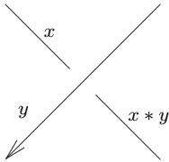
Figure 1: Definition of a coloring at a crossing
