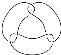
Figure 5: The 3-component link, whose exterior is the magic manifold
