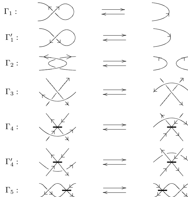
Figure 2: Yoshikawa moves of type I
