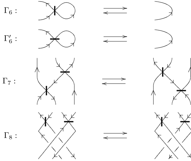
Figure 3: Yoshikawa moves of type II
