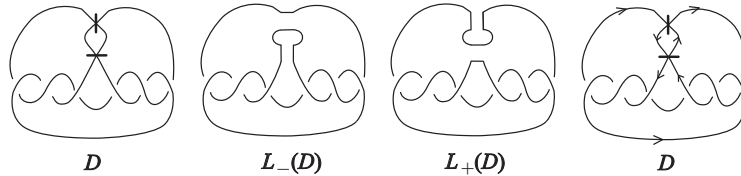
Figure 1: A marked graph diagram and its resolutions
