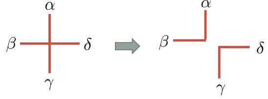
Figure 23: 2-dimensional matrix.
