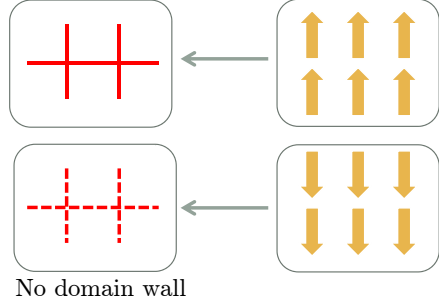
Figure 18: Up domain and down domain.
