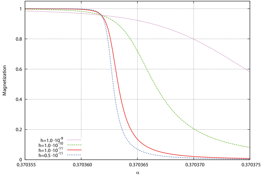
Figure 33: Magnetization versus temperature.
