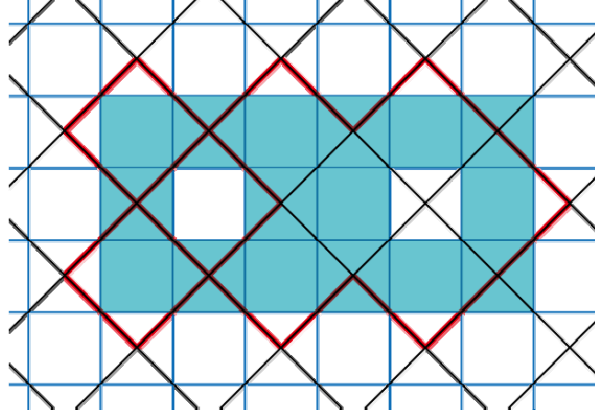
Figure 12: Coarse graining example.
