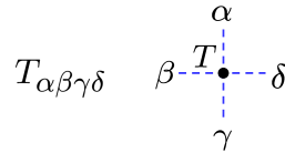
Figure 5: Vertex tensor.
