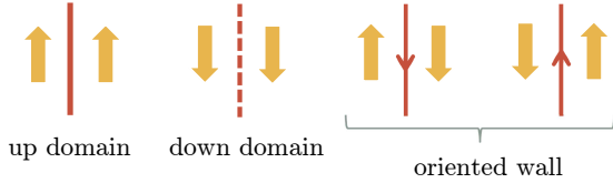
Figure 19: Four domain wall states.
