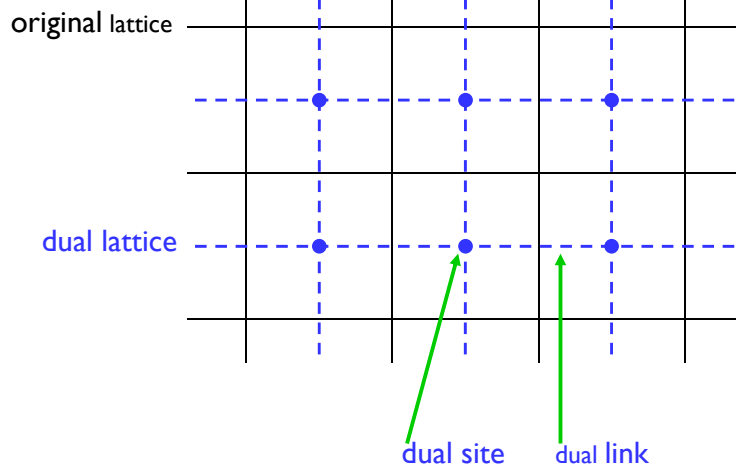
Figure 1: Dual lattice of the 2d square lattice.
