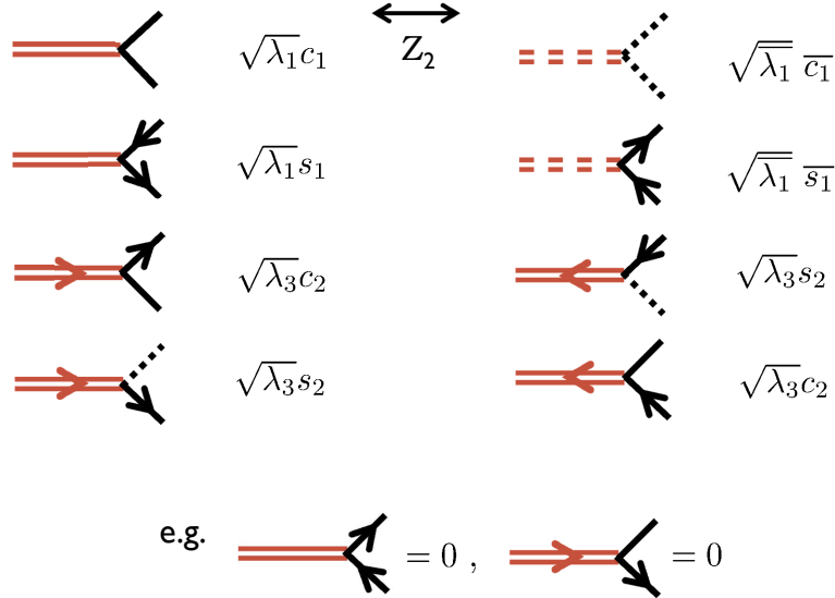
Figure 28: Feynman rules between micro and macro.
