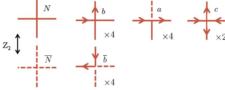
Figure 21: Non-vanishing 16 elements of the vertex tensor.
