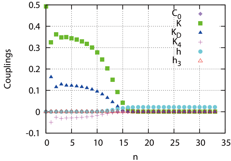
Figure 31: High temperature flow.
