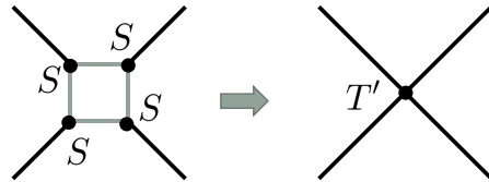
Figure 14: Renormalization of T .
