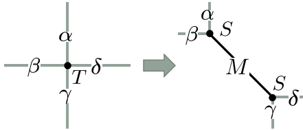
Figure 13: Splitting vertex T .
