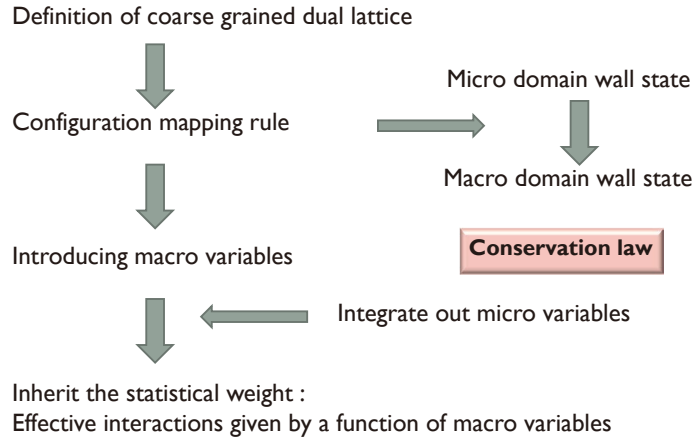
Figure 8: Domain wall renormalization group.
