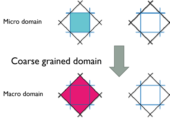
Figure 10: Definition of coarse grained domains.
