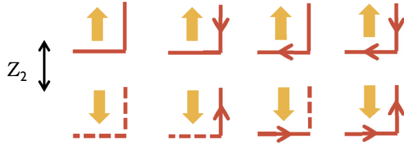
Figure 24: Non-vanishing indices.
