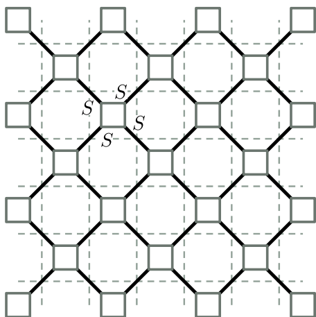
Figure 15: Global landscape 1.
