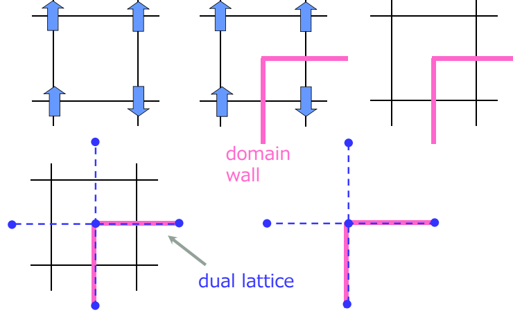
Figure 3: Domain wall representation of spin configuration.
