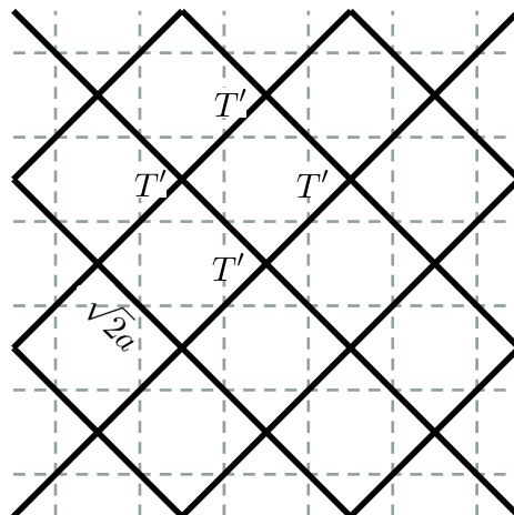
Figure 16: Global landscape 2.
