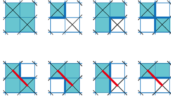
Figure 11: Macro domain walls and the mapping function.
