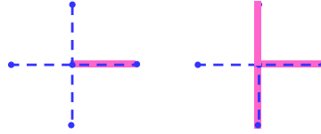
Figure 4: Prohibited non-conservative vertices.
