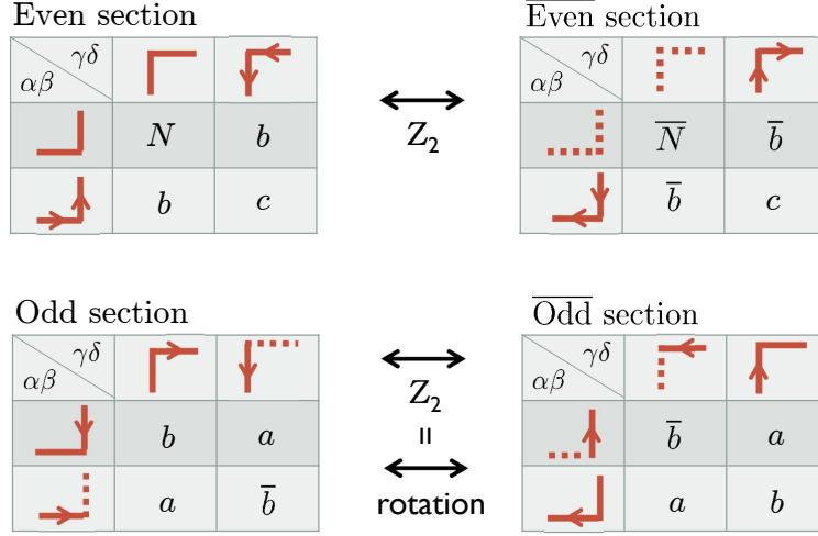
Figure 25: Even and odd section.
