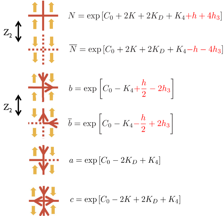
Figure 30: Transformation between spin and domain wall interactions.
