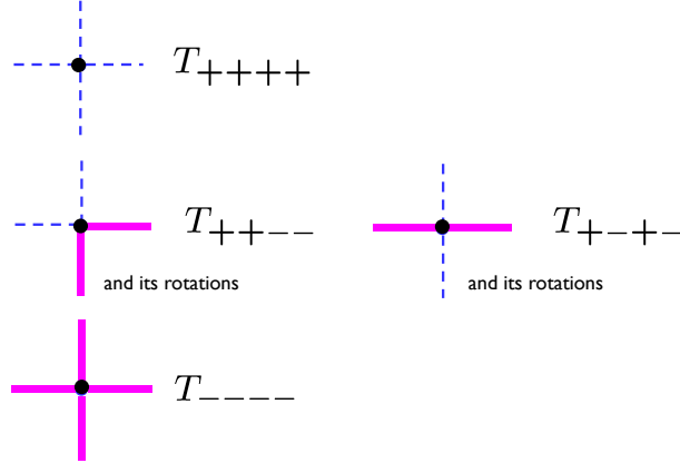
Figure 7: Non-vanishing elements of tensor.
