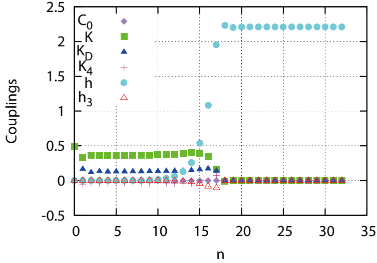
Figure 32: Low temperature flow.
