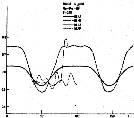
Fig. 5 Time changes of the mean velocity(U) and temperature( \Theta ) at z=0.75 level of the layer in the quasi-linear system. Time changes in the non-linear system are also shown.
