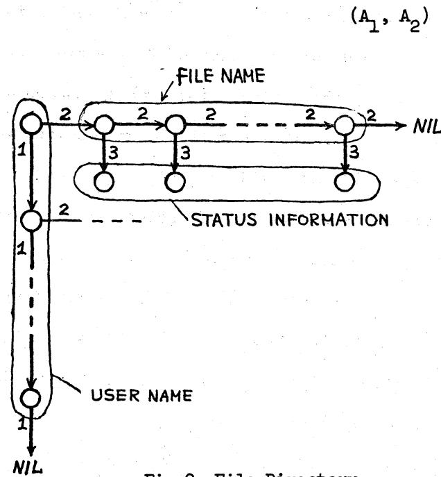
Fig.2. File Directory
