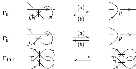
Figure 4: Moves of Type III
