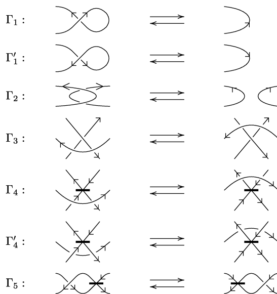
Figure 2: Moves of Type I
