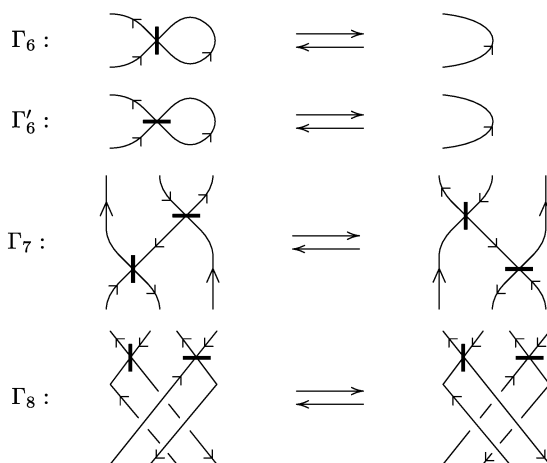
Figure 3: Moves of Type II
