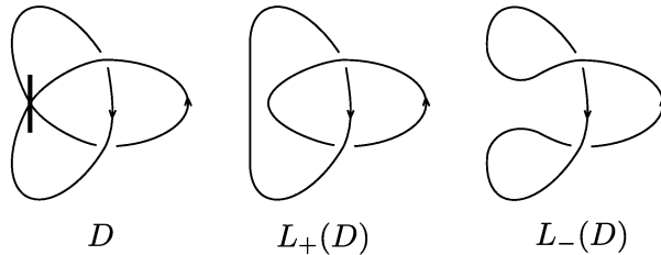
Figure 1: H-admissible marked graph diagram
