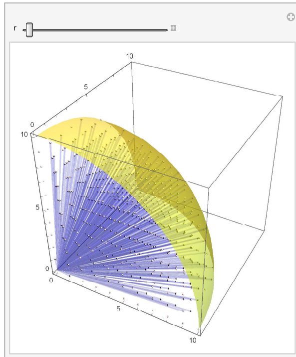
図 3: 3-dimensional case
