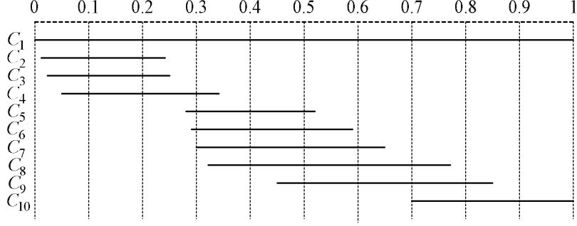
Figure 10: Players N = \{1, 2, \dots, 10\} and their valuation intervals C_1 = (0, 1] , C_2 = (0.01, 0.24] , C_3 = (0.02, 0.25] , C_4 = (0.05, 0.34] , C_5 = (0.28, 0.52] , C_6 = (0.29, 0.59] , C_7 = (0.3, 0.65] , C_8 = (0.32, 0.77] , C_9 = (0.45, 0.85] , C_{10} = (0.7, 1] . In this case, X = (0, 1] is a minimal interval of minimum density \rho_{\min} = 0.1 , and there are several separable intervals of X = (0, 1] such as (0.01, 0.25] , (0.01, 0.59] , (0.01, 1] , (0.28, 0.65] , (0.28, 0.77] , (0.28, 0.85] . The largest left endpoint y^* of the separable intervals in X is 0.28 and the set of separable intervals with the largest left endpoint y^* = 0.28 is \{(0.28, 0.65], (0.28, 0.77], (0.28, 0.85)\} .
