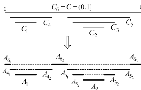
Figure 4: An allocated piece to player 5 is \{A_{5_1}, A_{5_2}\} ( n = 6 ). \text{csize}(A_6) = \text{csize}(A_{6_1}) + \text{csize}(A_{6_2}) + \text{csize}(A_{6_3}) for A_6 = A_{6_1} + A_{6_2} + A_{6_3} .
