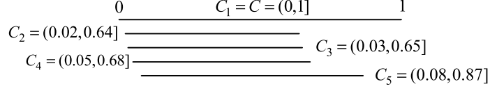
Figure 1: An input example for the cake-cutting problem ( n = 5 ). Player 1 is allocated (0, 0.07] \cup (0.87, 1] , player 2 is allocated (0.07, 0.27] , player 3 is allocated (0.27, 0.47] , player 4 is allocated (0.47, 0.67] and player 5 is allocated (0.67, 0.87] .
