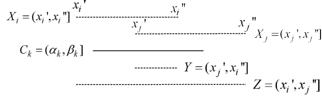
Figure 7: Two intervals X_i = (x_i', x_i''] and X_j = (x_j', x_j''] in Proof of Lemma 4.1. A valuation interval C_k = (\alpha_k, \beta_k] is not in X_i nor X_j , but in Z = X_i \cup X_j .
