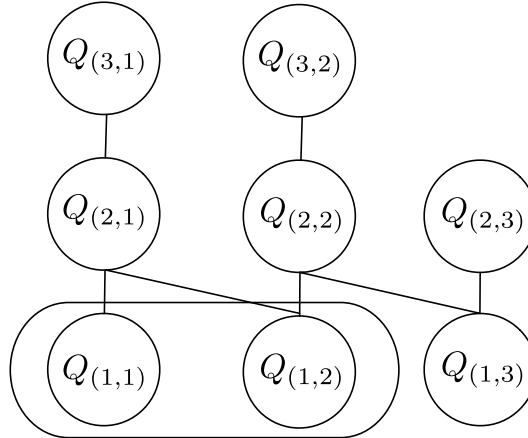
図 3: MIS-localization
