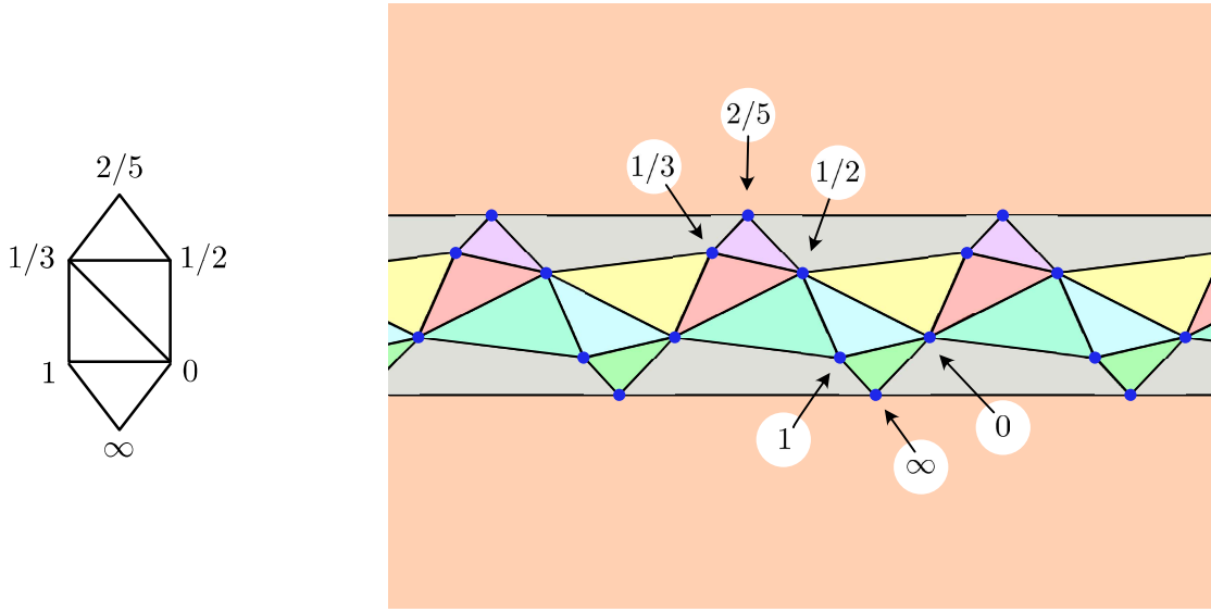
Figure 4: The facial structure of T_a
