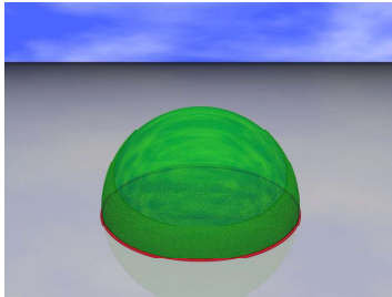
Figure 1: Isometric hemisphere: the underlying space of the upper half space model for \mathbb{H}^3 is the upper half space of \mathbb{R}^3 , whose ideal boundary is identified with the one-point compactification \widehat{\mathbb{C}} of the horizontal plane of height 0 identified with \mathbb{C} .
