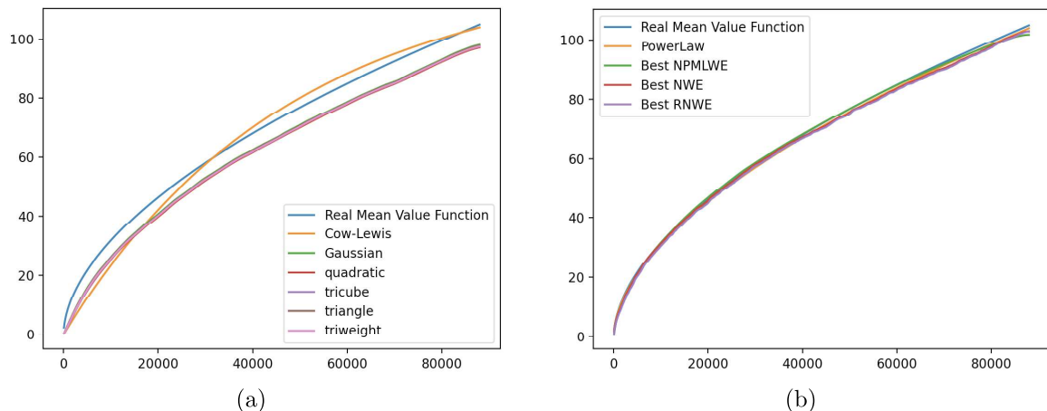
Figure 2: Estimation of the cumulative number of failures/minimal repairs.
