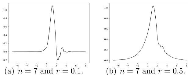
Figure 1: Positive basis functions.
