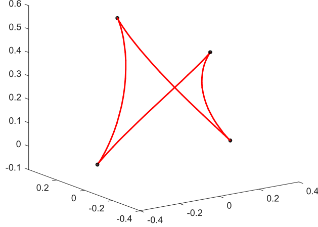
Figure 1: A null type curve with four singularities.
