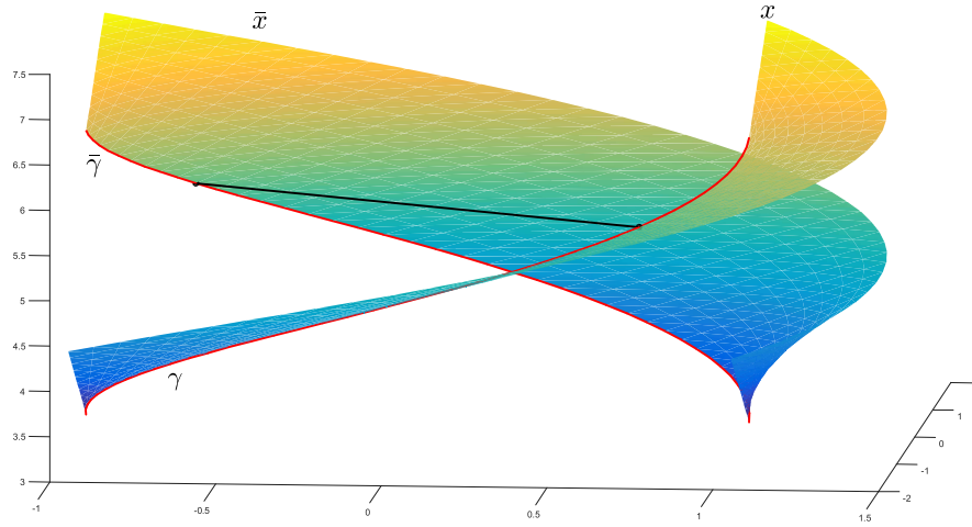
Figure 4: \boldsymbol{x} and its Bertrand offset \bar{\boldsymbol{x}} in Example 5.2.
