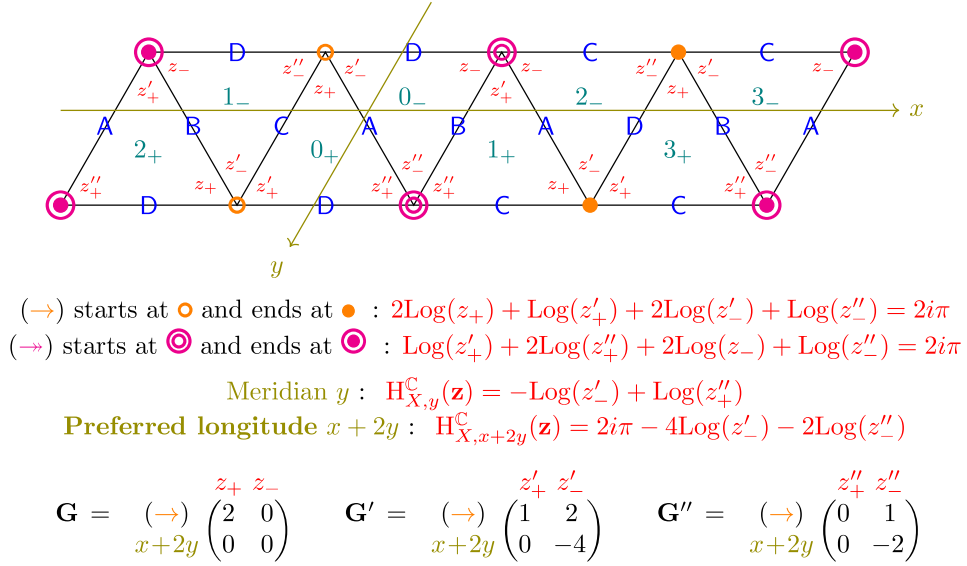
Figure 2: Cusp triangulation of S^3 \setminus 4_1 , and the Neumann–Zagier matrices
