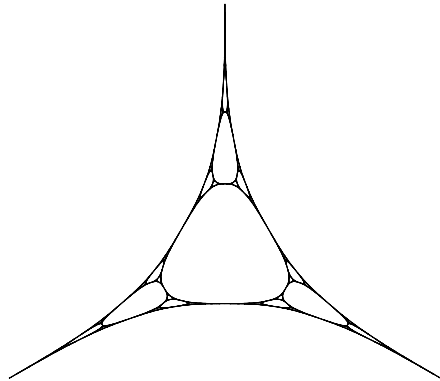
FIGURE 2. Harmonic Sierpiński gasket
