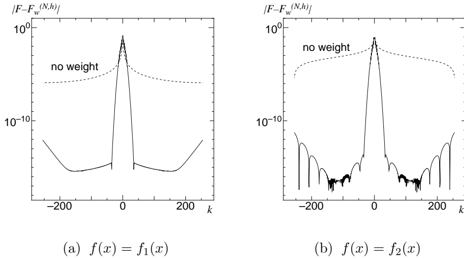
図 6: Fourier 変換の近似誤差 : F_w^{(N,h)}(\frac{2\pi}{Nh}k) , N = 512 , h = 0.125
